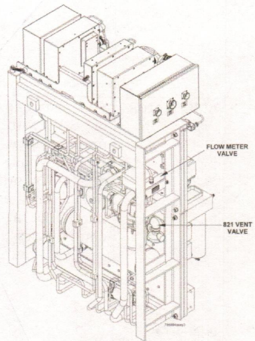
Rear View of CCB Panel
