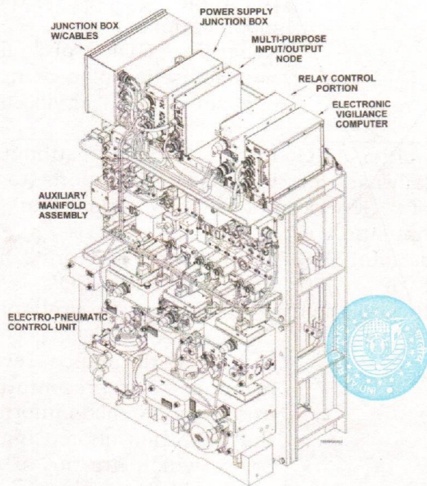
Front view of CCB Panel
